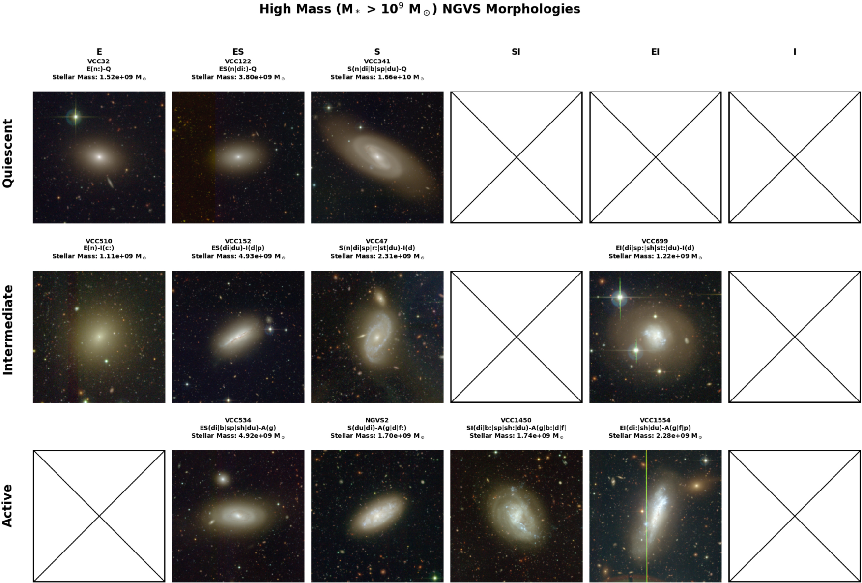
Figure 1. from Max M. Kurzner et al 2025 Astron. J. 170 doi:10.3847/1538-3881/ae1616 https://dx.doi.org/10.3847/1538-3881/ae1616 © 2025. The Author(s). Published by the American Astronomical Society.
