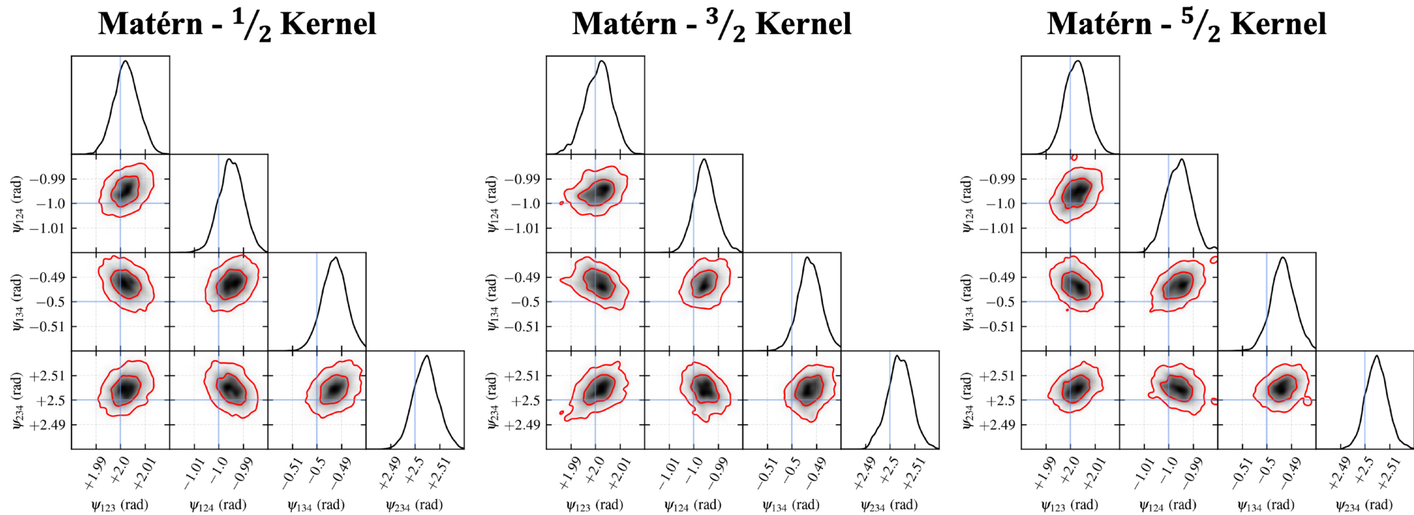
Figure 7. from Uri Rolls et al 2026 Astron. J. 171 doi:10.3847/1538-3881/ae160f https://dx.doi.org/10.3847/1538-3881/ae160f © 2025. The Author(s). Published by the American Astronomical Society.
