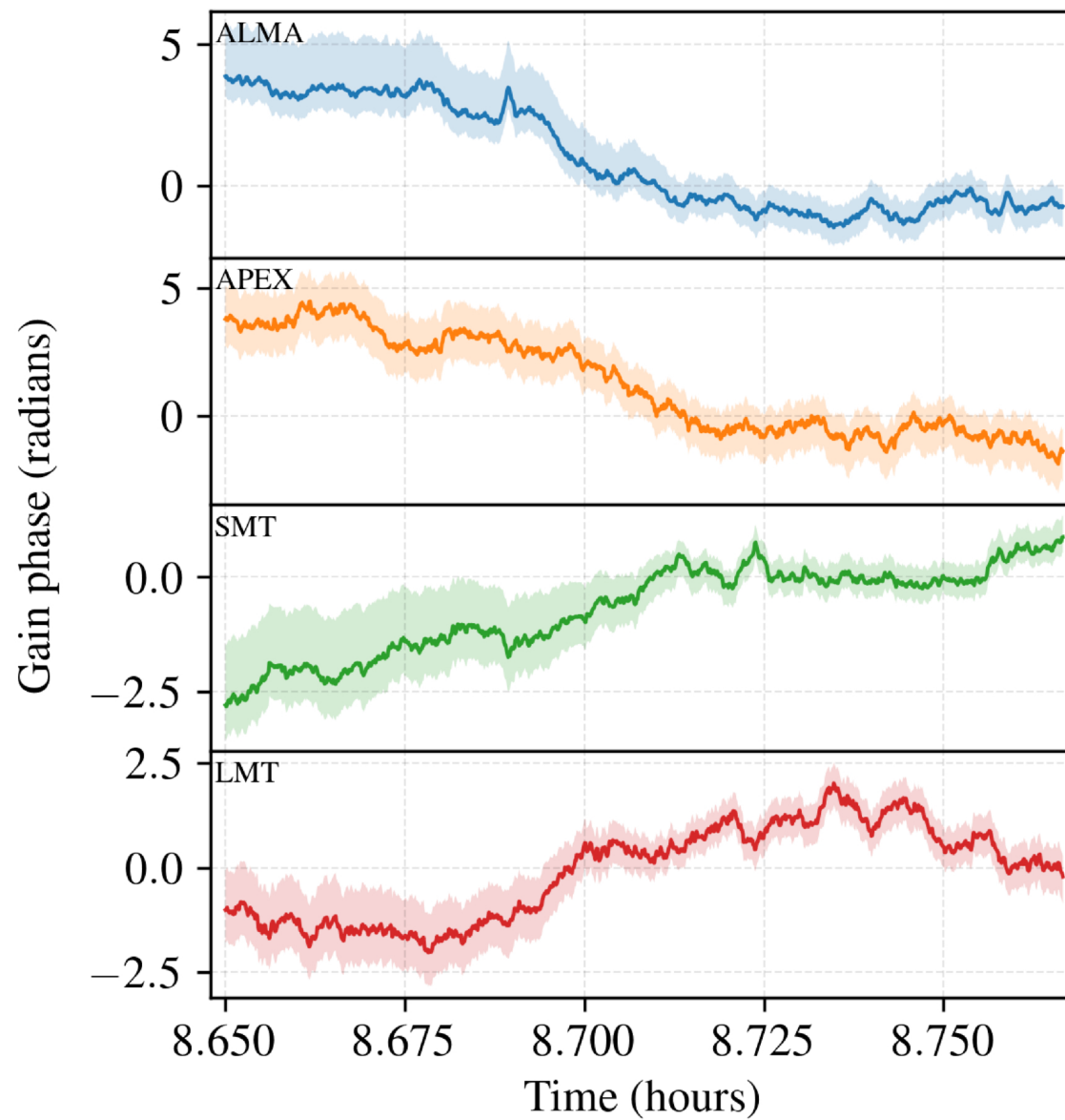
Figure 5. from Uri Rolls et al 2026 Astron. J. 171 doi:10.3847/1538-3881/ae160f https://dx.doi.org/10.3847/1538-3881/ae160f © 2025. The Author(s). Published by the American Astronomical Society.
