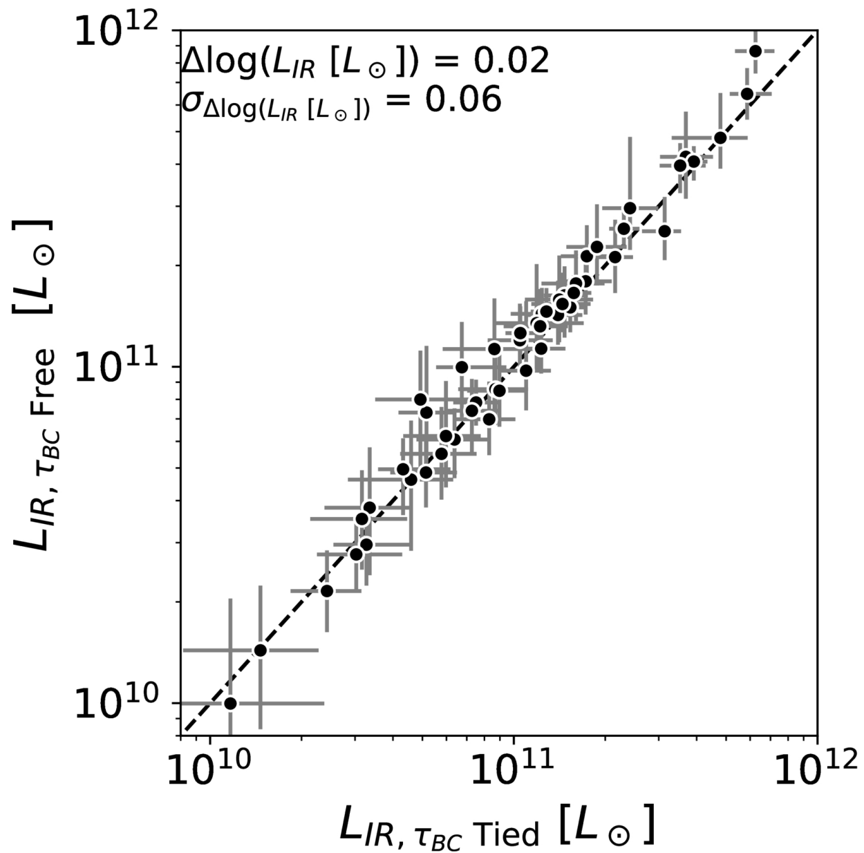
Figure 9. from David J. Setton et al 2025 Astron. J. 170 doi:10.3847/1538-3881/ae1607 https://dx.doi.org/10.3847/1538-3881/ae1607 © 2025. The Author(s). Published by the American Astronomical Society.
