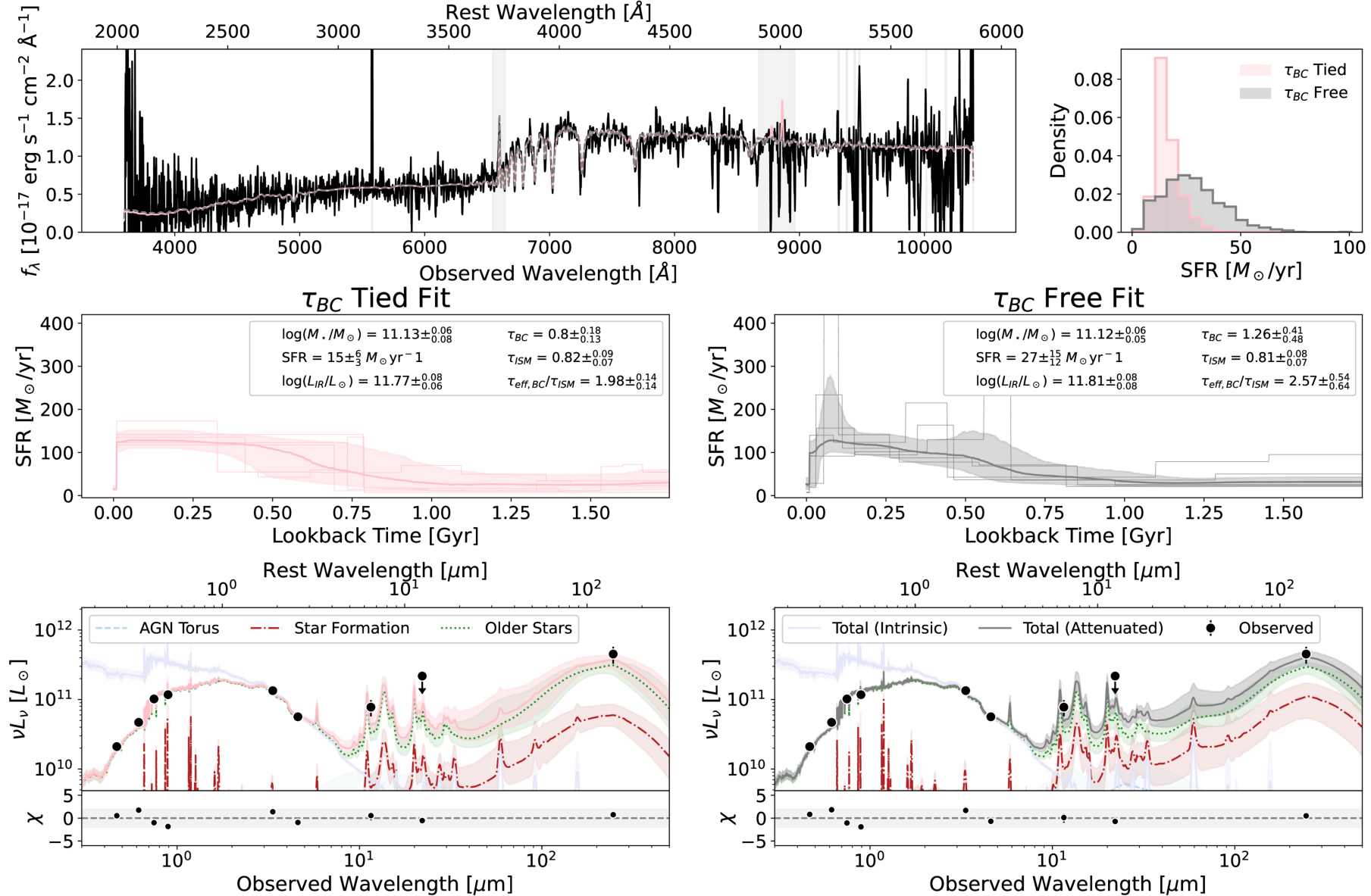
Figure 7. from David J. Setton et al 2025 Astron. J. 170 doi:10.3847/1538-3881/ae1607 https://dx.doi.org/10.3847/1538-3881/ae1607 © 2025. The Author(s). Published by the American Astronomical Society.
