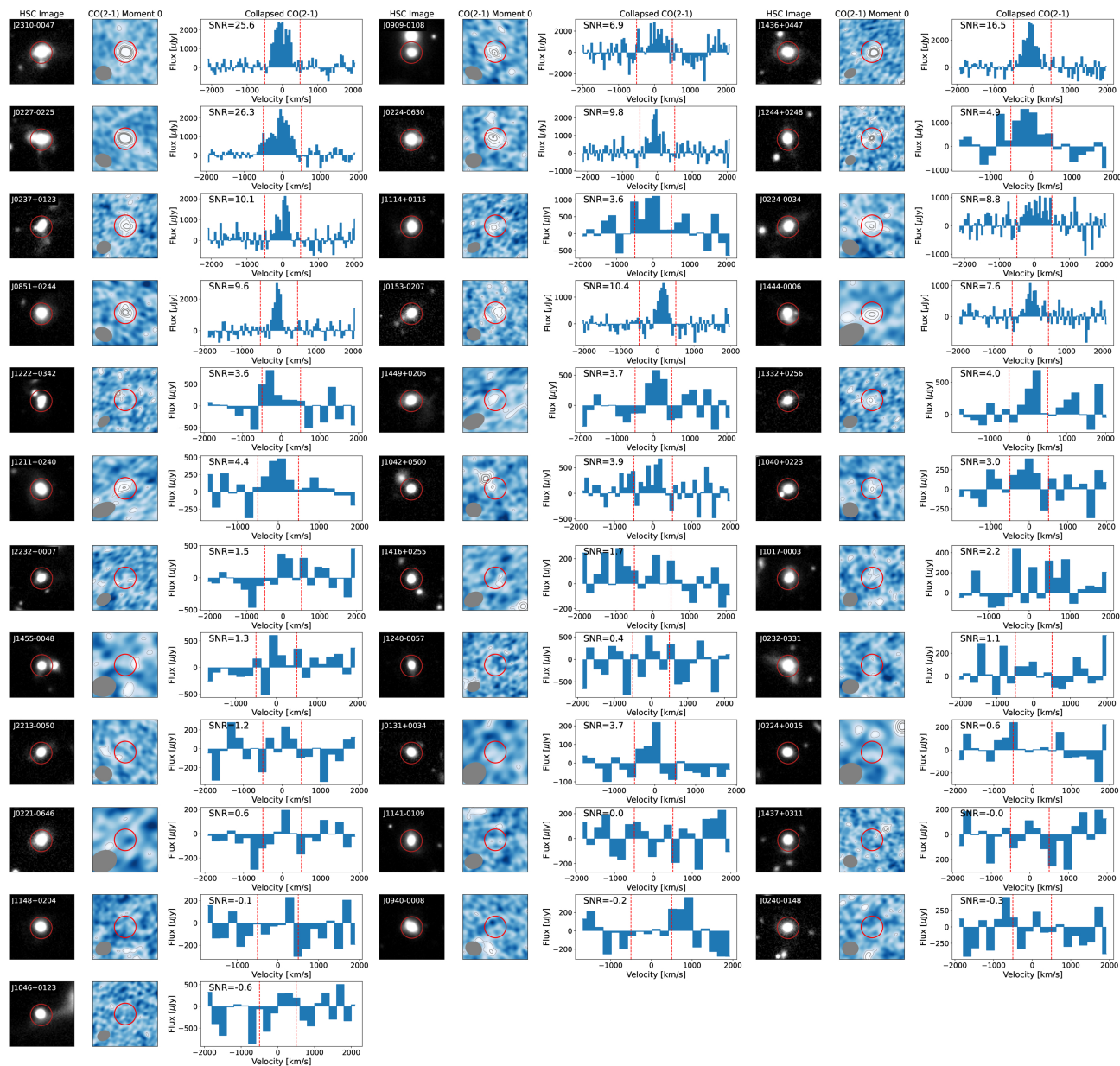
Figure 3. from David J. Setton et al 2025 Astron. J. 170 doi:10.3847/1538-3881/ae1607 https://dx.doi.org/10.3847/1538-3881/ae1607 © 2025. The Author(s). Published by the American Astronomical Society.
