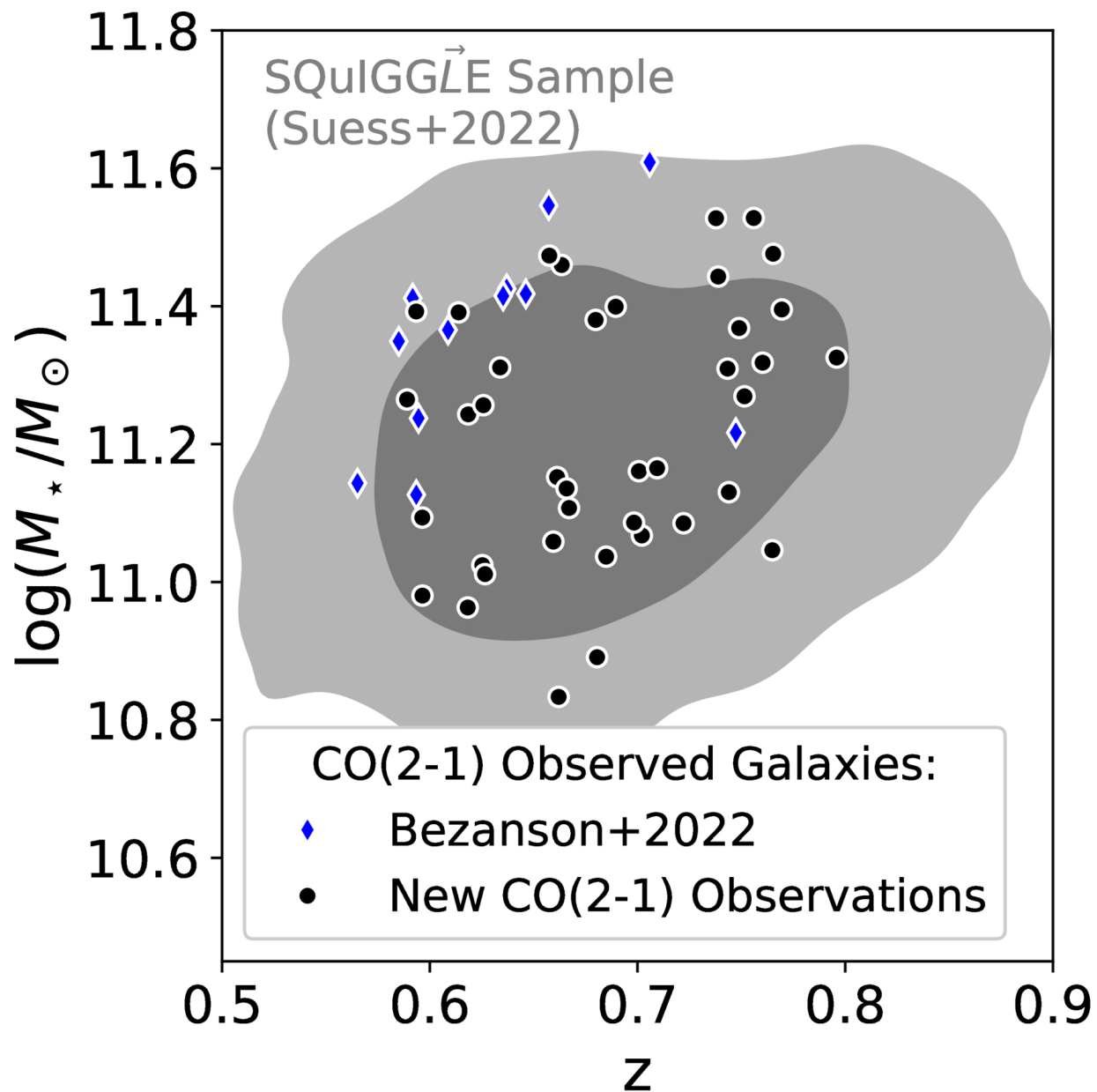
Figure 1. from David J. Setton et al 2025 Astron. J. 170 doi:10.3847/1538-3881/ae1607 https://dx.doi.org/10.3847/1538-3881/ae1607 © 2025. The Author(s). Published by the American Astronomical Society.
