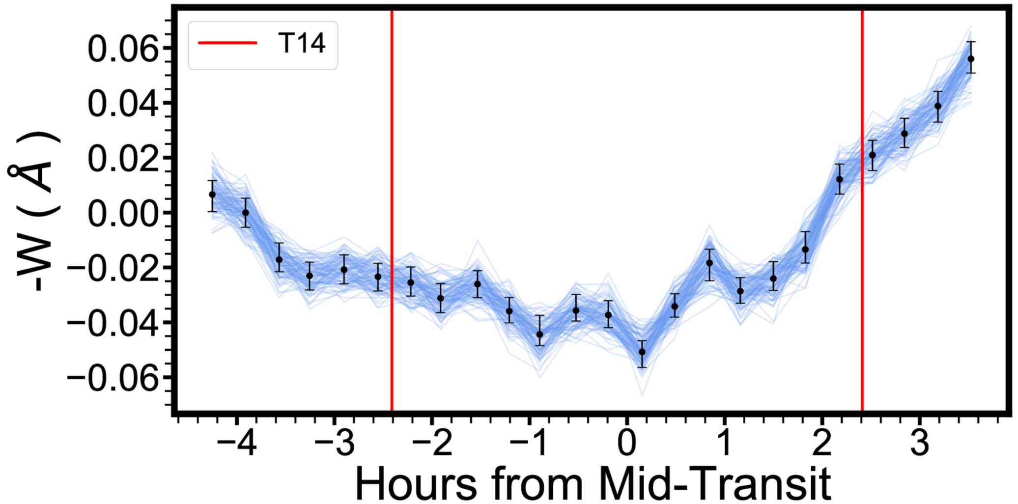
Figure 9. from Reilly P. Milburn et al 2025 Astron. J. 170 doi:10.3847/1538-3881/ae1504 https://dx.doi.org/10.3847/1538-3881/ae1504 © 2025. The Author(s). Published by the American Astronomical Society.
