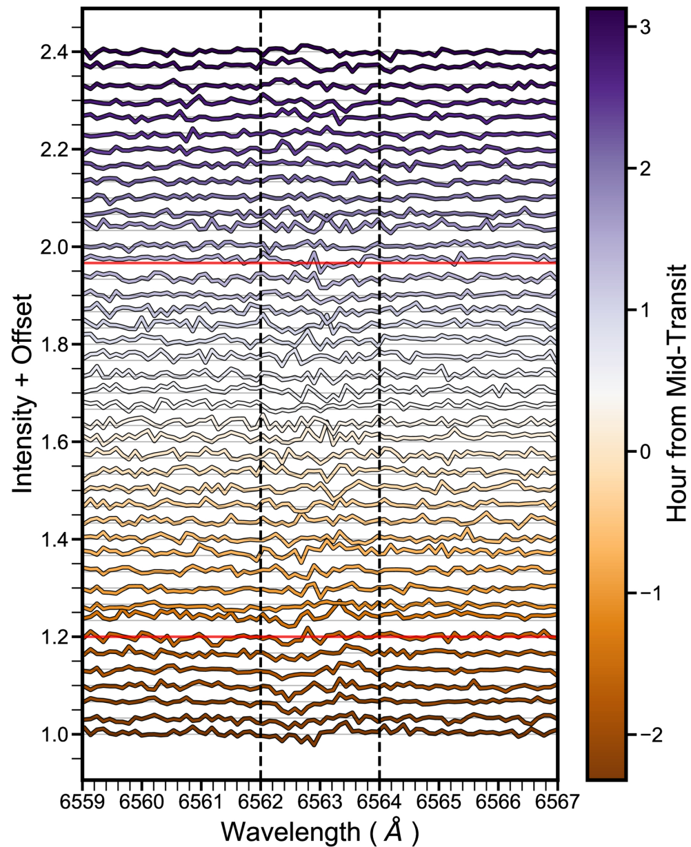
Figure 6. from Reilly P. Milburn et al 2025 Astron. J. 170 doi:10.3847/1538-3881/ae1504 https://dx.doi.org/10.3847/1538-3881/ae1504 © 2025. The Author(s). Published by the American Astronomical Society.
