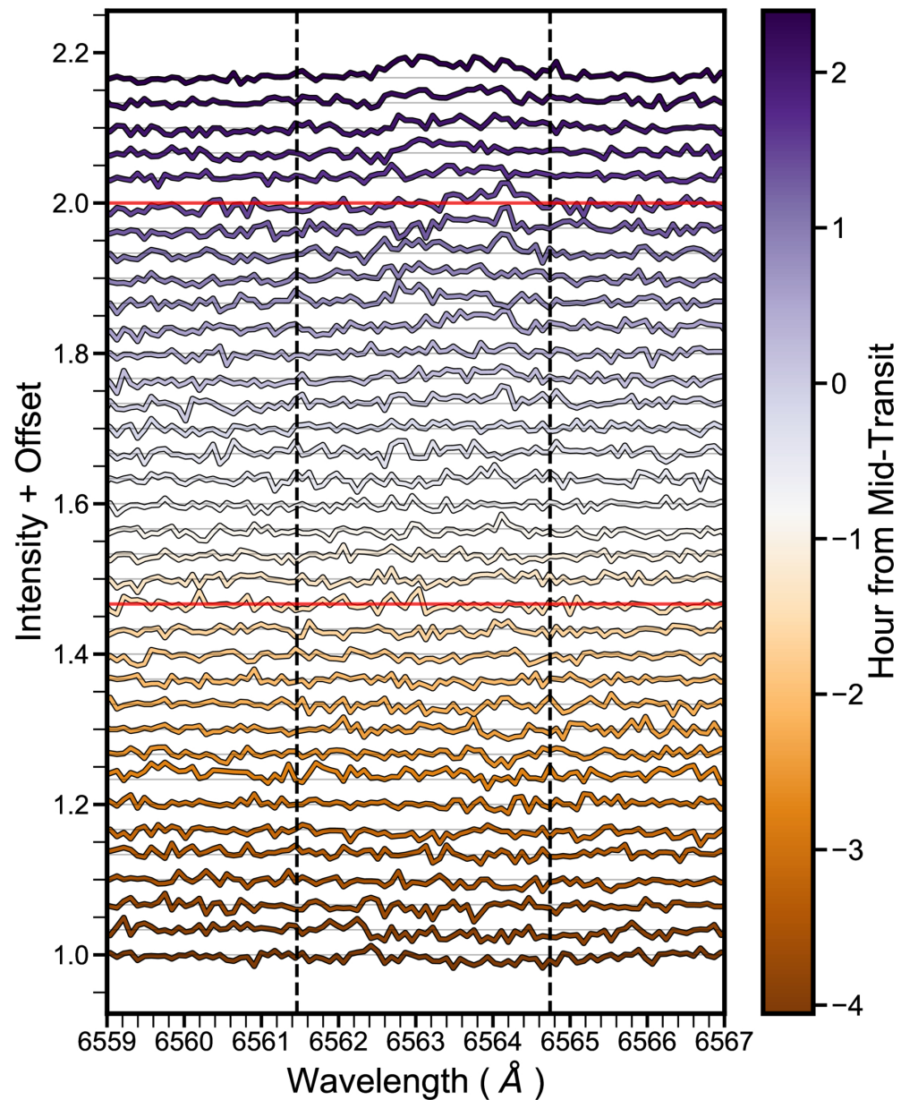
Figure 5. from Reilly P. Milburn et al 2025 Astron. J. 170 doi:10.3847/1538-3881/ae1504 https://dx.doi.org/10.3847/1538-3881/ae1504 © 2025. The Author(s). Published by the American Astronomical Society.
