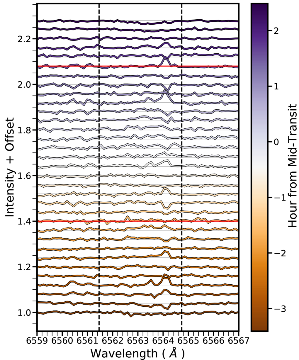
Figure 4. from Reilly P. Milburn et al 2025 Astron. J. 170 doi:10.3847/1538-3881/ae1504 https://dx.doi.org/10.3847/1538-3881/ae1504 © 2025. The Author(s). Published by the American Astronomical Society.
