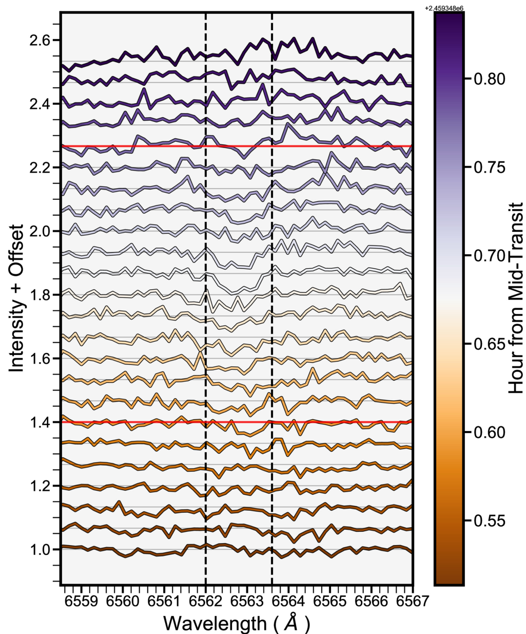
Figure 3. from Reilly P. Milburn et al 2025 Astron. J. 170 doi:10.3847/1538-3881/ae1504 https://dx.doi.org/10.3847/1538-3881/ae1504 © 2025. The Author(s). Published by the American Astronomical Society.
