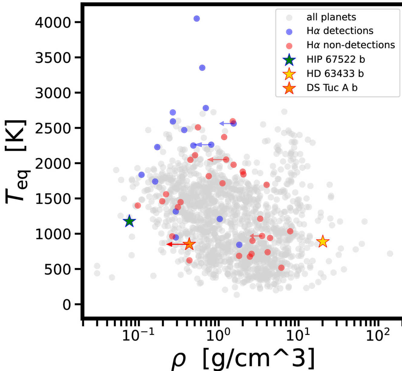
Figure 15. from Reilly P. Milburn et al 2025 Astron. J. 170 doi:10.3847/1538-3881/ae1504 https://dx.doi.org/10.3847/1538-3881/ae1504 © 2025. The Author(s). Published by the American Astronomical Society.
