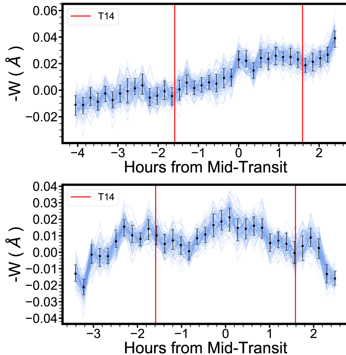
Figure 14. from Reilly P. Milburn et al 2025 Astron. J. 170 doi:10.3847/1538-3881/ae1504 https://dx.doi.org/10.3847/1538-3881/ae1504 © 2025. The Author(s). Published by the American Astronomical Society.
