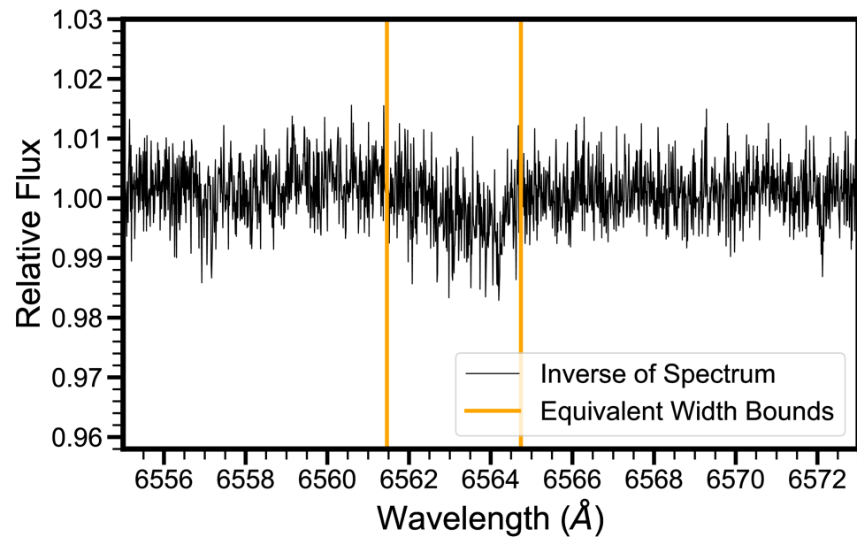
Figure 13. from Reilly P. Milburn et al 2025 Astron. J. 170 doi:10.3847/1538-3881/ae1504 https://dx.doi.org/10.3847/1538-3881/ae1504 © 2025. The Author(s). Published by the American Astronomical Society.
