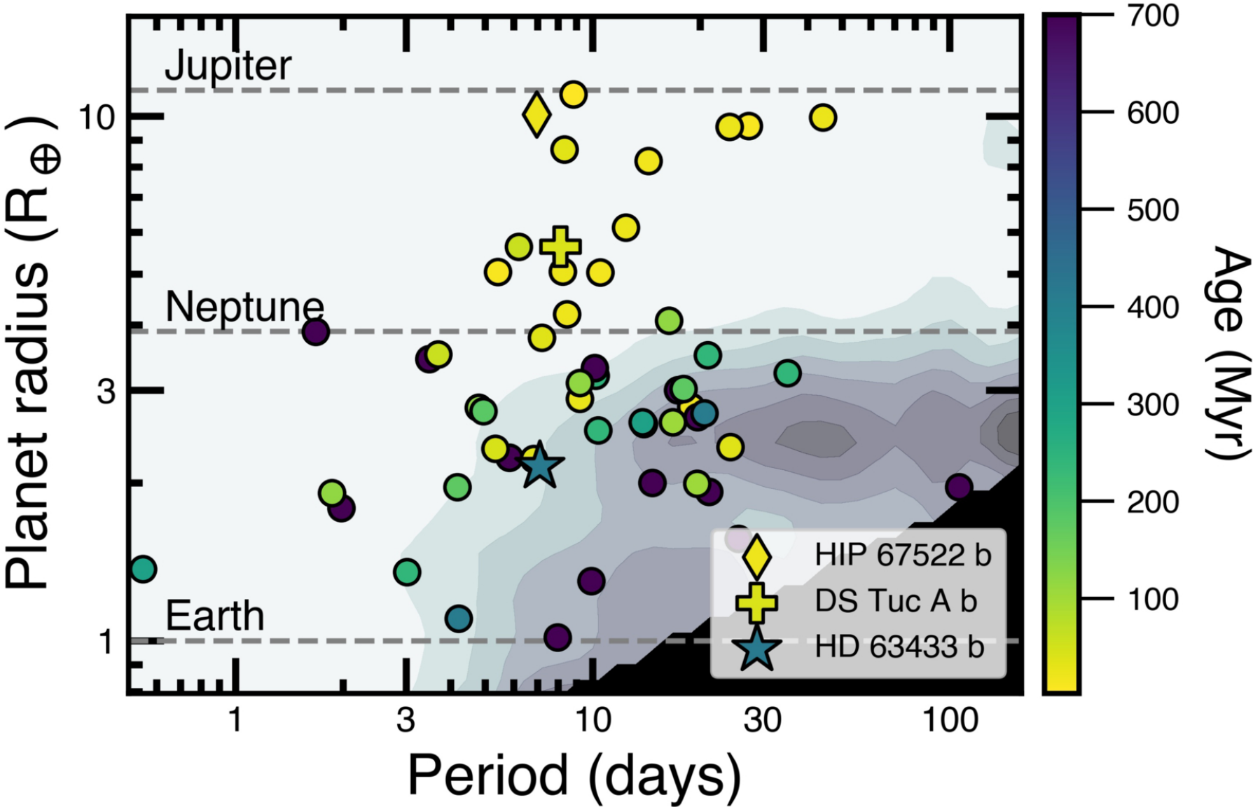
Figure 1. from Reilly P. Milburn et al 2025 Astron. J. 170 doi:10.3847/1538-3881/ae1504 https://dx.doi.org/10.3847/1538-3881/ae1504 © 2025. The Author(s). Published by the American Astronomical Society.
