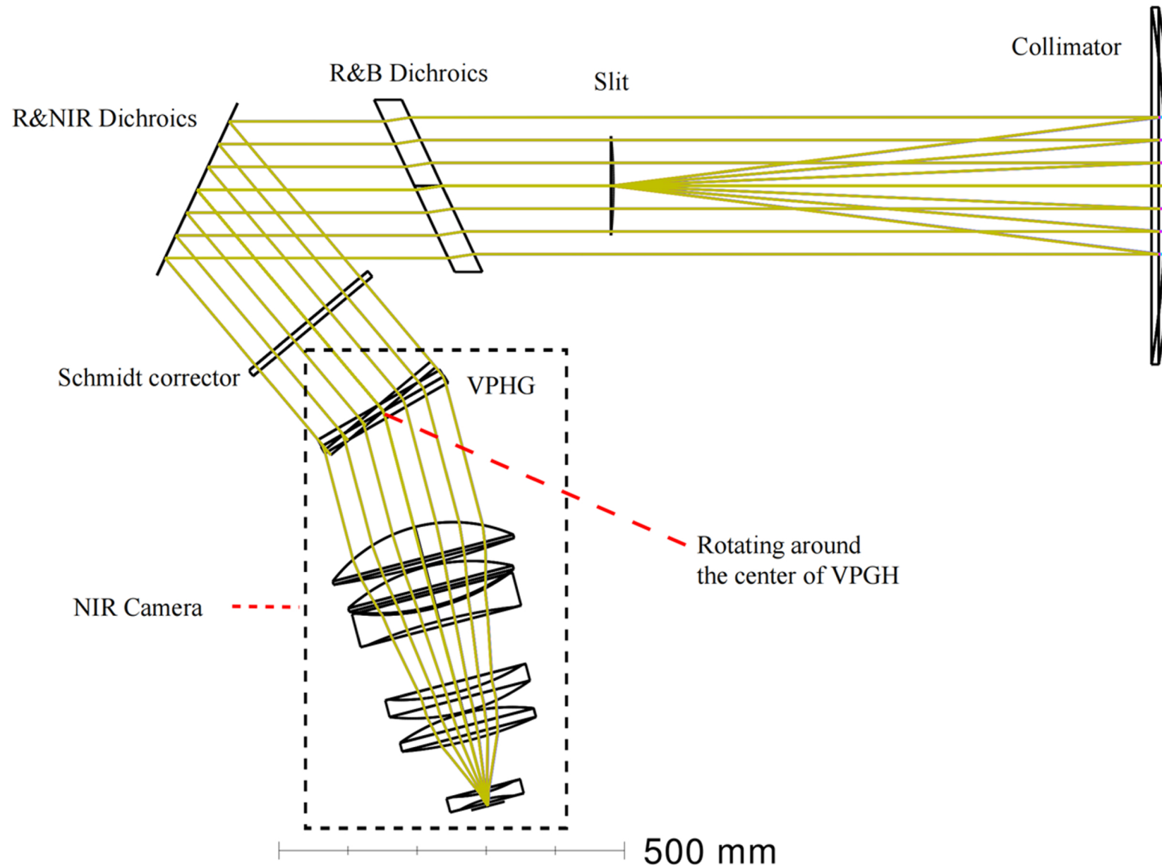
Figure 7. from Xiaojie Zhang et al 2025 Astron. J. 170 doi:10.3847/1538-3881/ae14f8 https://dx.doi.org/10.3847/1538-3881/ae14f8 © 2025. The Author(s). Published by the American Astronomical Society.
