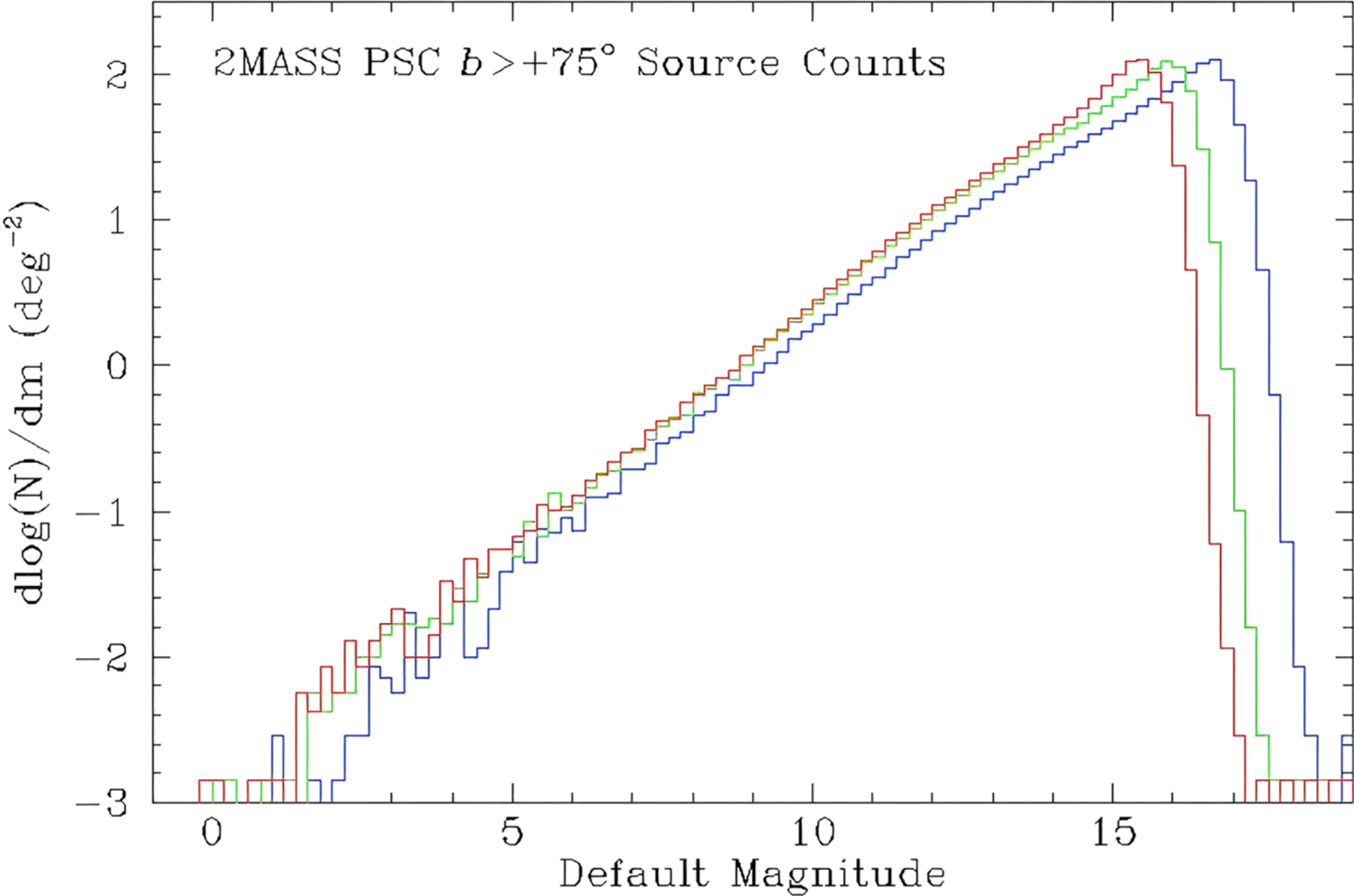
Figure 3. from Xiaojie Zhang et al 2025 Astron. J. 170 doi:10.3847/1538-3881/ae14f8 https://dx.doi.org/10.3847/1538-3881/ae14f8 © 2025. The Author(s). Published by the American Astronomical Society.
