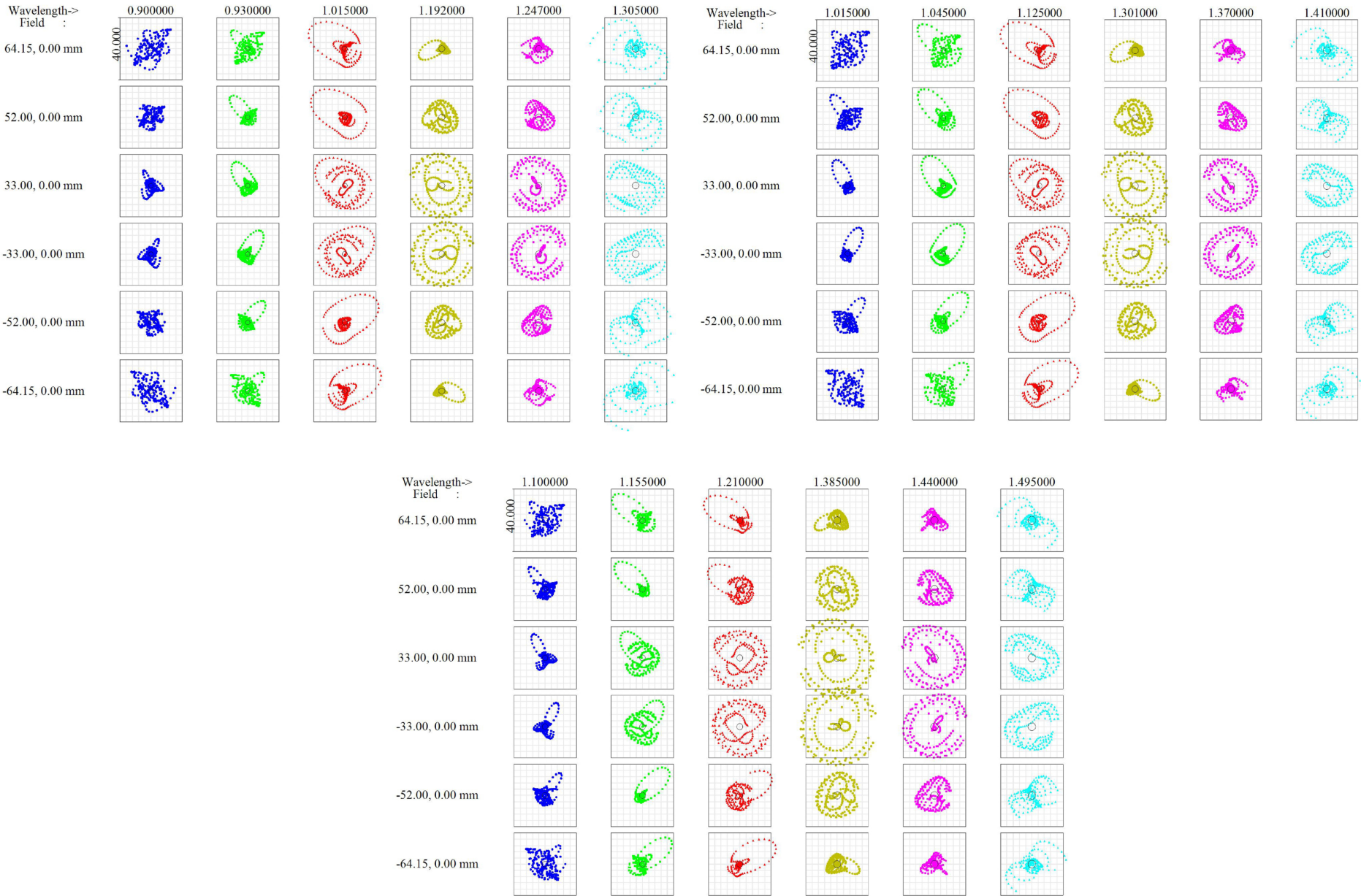
Figure 10. from Xiaojie Zhang et al 2025 Astron. J. 170 doi:10.3847/1538-3881/ae14f8 https://dx.doi.org/10.3847/1538-3881/ae14f8 © 2025. The Author(s). Published by the American Astronomical Society.
