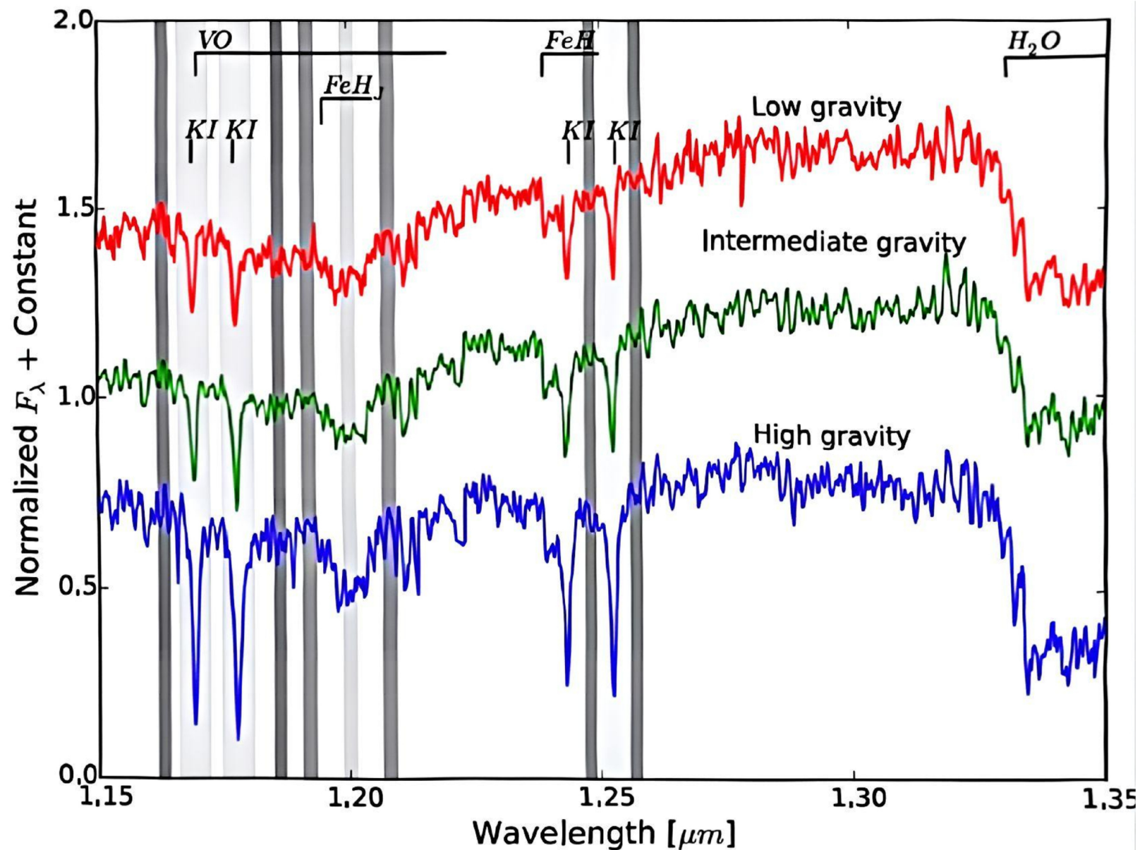
Figure 1. from Xiaojie Zhang et al 2025 Astron. J. 170 doi:10.3847/1538-3881/ae14f8 https://dx.doi.org/10.3847/1538-3881/ae14f8 © 2025. The Author(s). Published by the American Astronomical Society.
