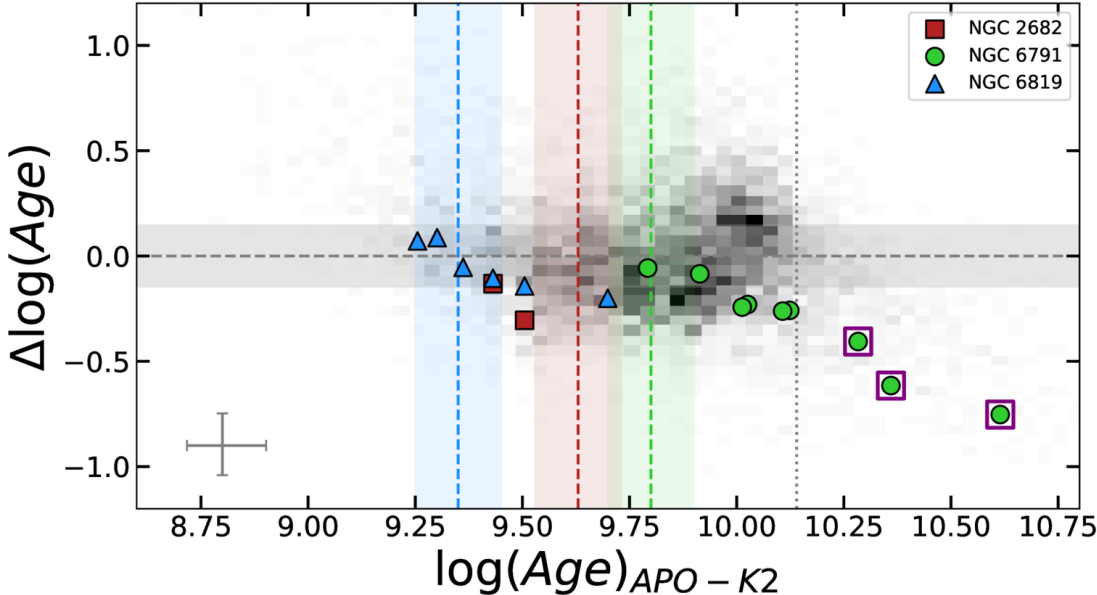
Figure 11. from Taylor Spoo et al 2025 Astron. J. 170 doi:10.3847/1538-3881/ae14ec https://dx.doi.org/10.3847/1538-3881/ae14ec © 2025. The Author(s). Published by the American Astronomical Society.
