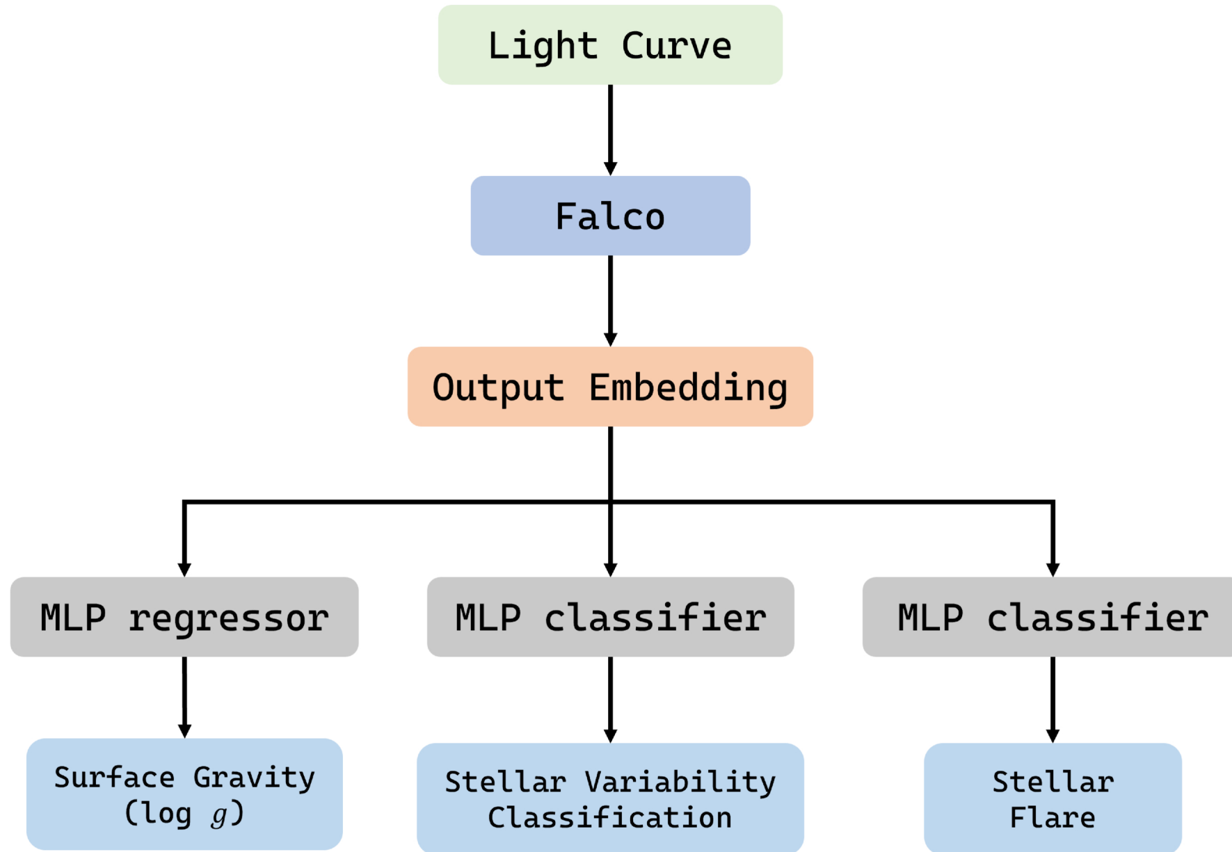
Figure 5. from Xiaoxiong Zuo et al 2026 Astron. J. 171 doi:10.3847/1538-3881/ae1467 https://dx.doi.org/10.3847/1538-3881/ae1467 © 2025. The Author(s). Published by the American Astronomical Society.
