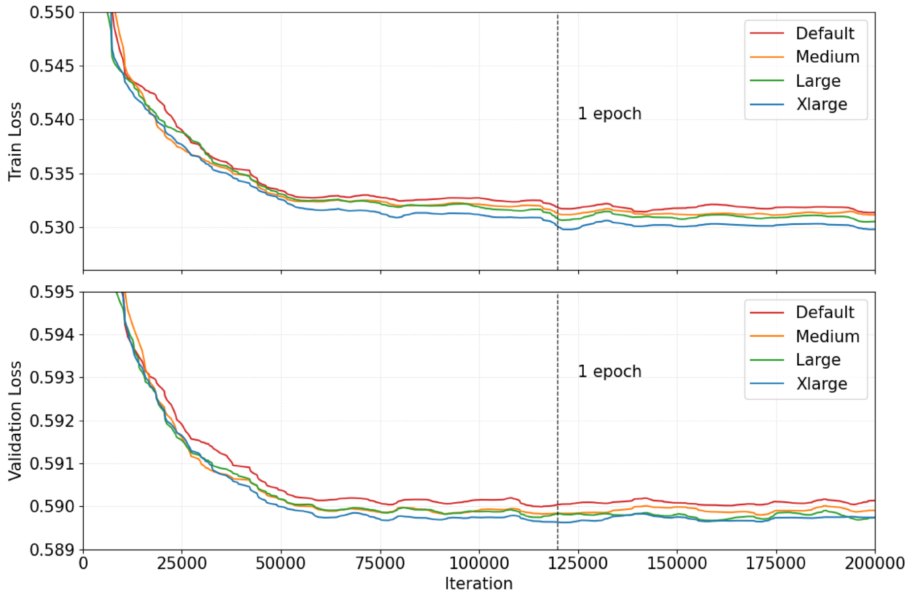
Figure 4. from Xiaoxiong Zuo et al 2026 Astron. J. 171 doi:10.3847/1538-3881/ae1467 https://dx.doi.org/10.3847/1538-3881/ae1467 © 2025. The Author(s). Published by the American Astronomical Society.
