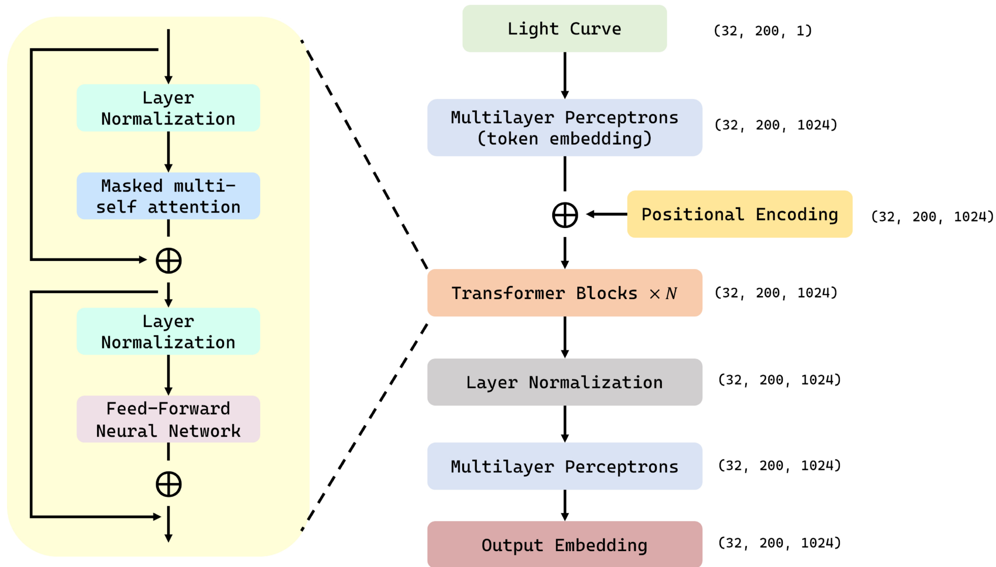
Figure 3. from Xiaoxiong Zuo et al 2026 Astron. J. 171 doi:10.3847/1538-3881/ae1467 https://dx.doi.org/10.3847/1538-3881/ae1467 © 2025. The Author(s). Published by the American Astronomical Society.
