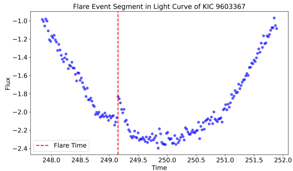
Figure 2. from Xiaoxiong Zuo et al 2026 Astron. J. 171 doi:10.3847/1538-3881/ae1467 https://dx.doi.org/10.3847/1538-3881/ae1467 © 2025. The Author(s). Published by the American Astronomical Society.
