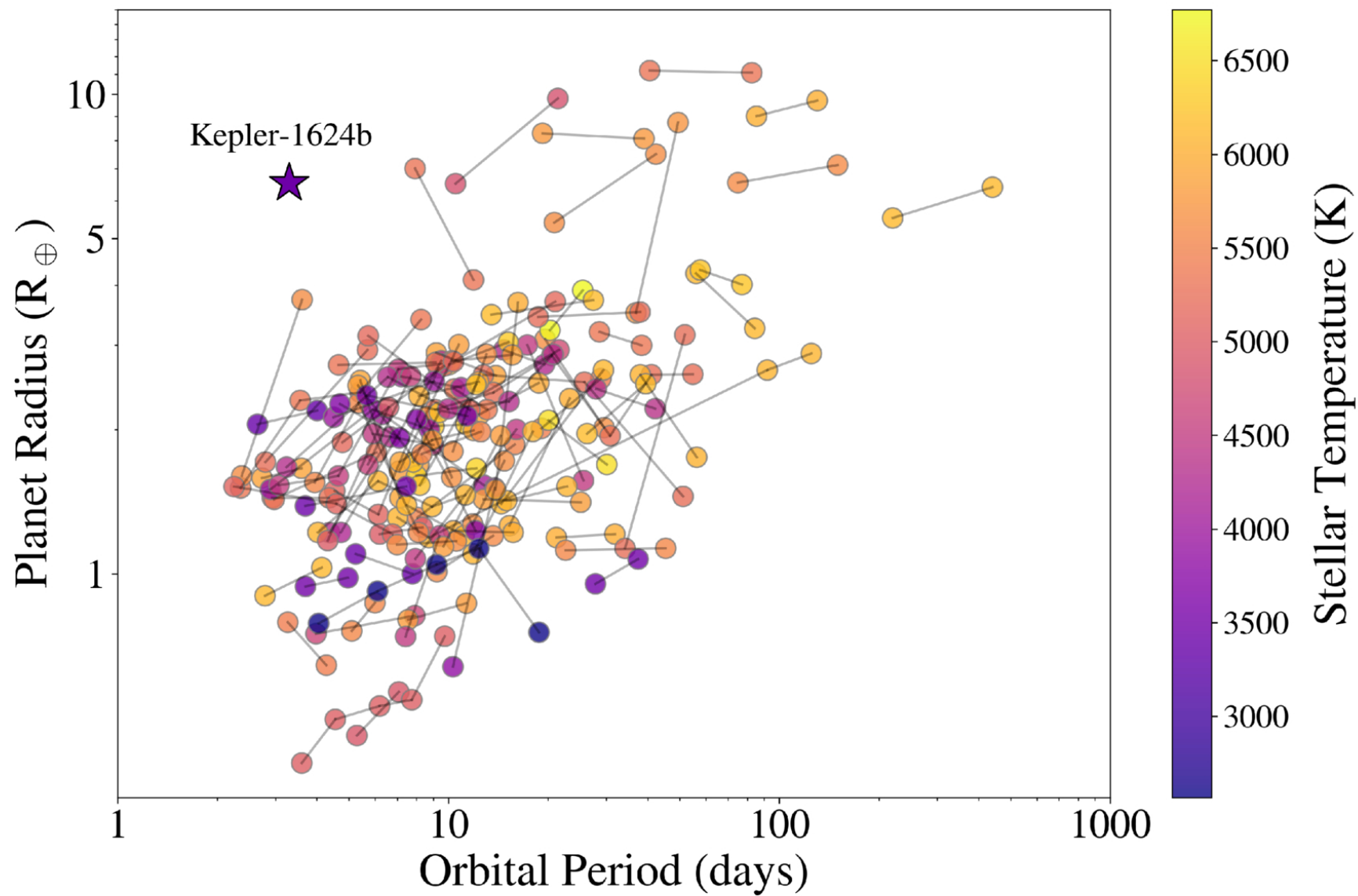
Figure 1. from Haedam Im et al 2025 Astron. J. 170 doi:10.3847/1538-3881/ae1464 https://dx.doi.org/10.3847/1538-3881/ae1464 © 2025. The Author(s). Published by the American Astronomical Society.
