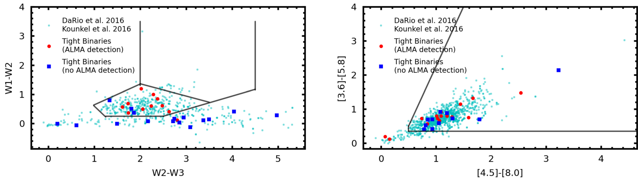
Figure 6. from Kevin Flaherty et al 2025 Astron. J. 170 doi:10.3847/1538-3881/ae112b https://dx.doi.org/10.3847/1538-3881/ae112b © 2025. The Author(s). Published by the American Astronomical Society.
