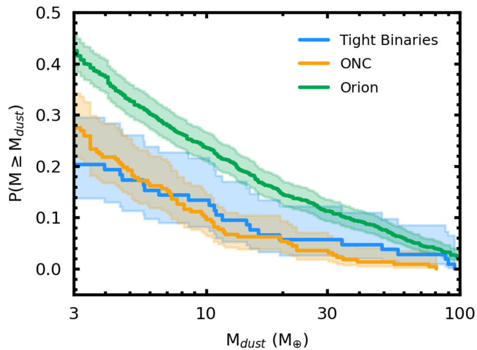
Figure 5. from Kevin Flaherty et al 2025 Astron. J. 170 doi:10.3847/1538-3881/ae112b https://dx.doi.org/10.3847/1538-3881/ae112b © 2025. The Author(s). Published by the American Astronomical Society.
