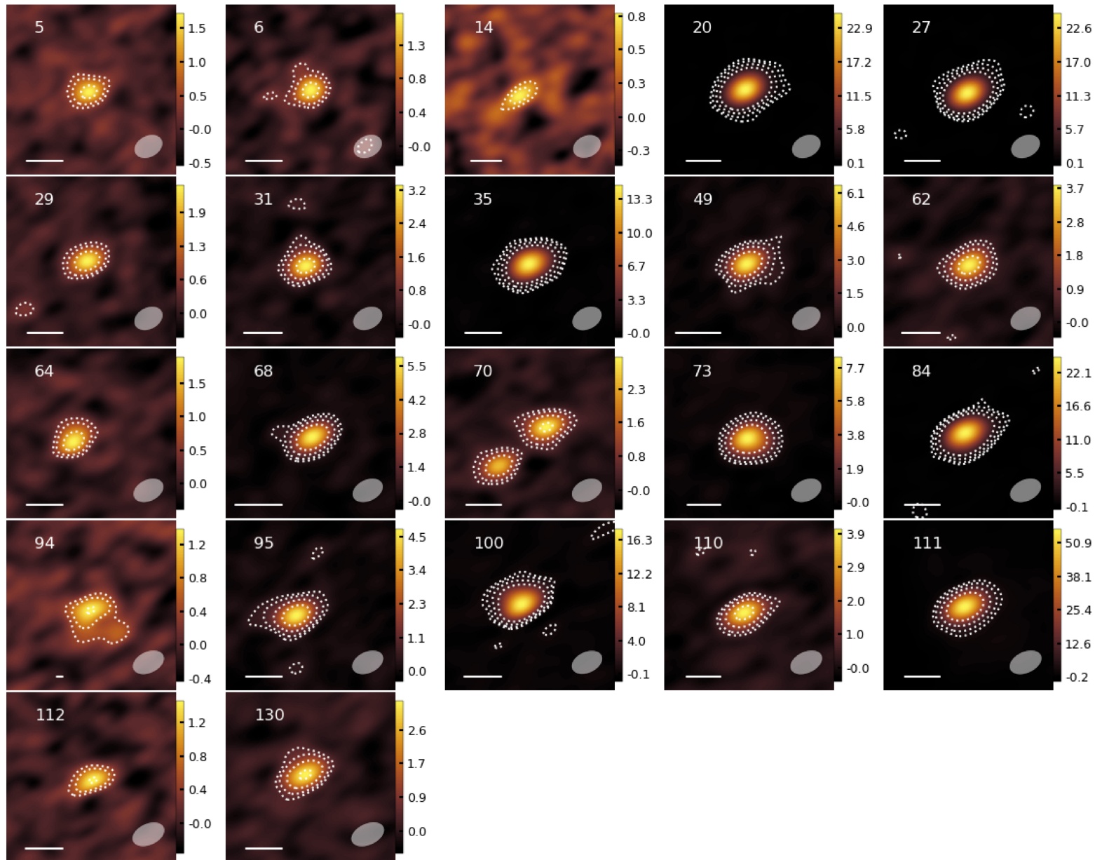
Figure 2. from Kevin Flaherty et al 2025 Astron. J. 170 doi:10.3847/1538-3881/ae112b https://dx.doi.org/10.3847/1538-3881/ae112b © 2025. The Author(s). Published by the American Astronomical Society.
