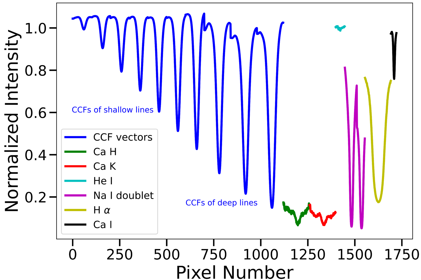
Figure 5. from Anoop Gavankar et al 2026 Astron. J. 171 doi:10.3847/1538-3881/ae11115 https://dx.doi.org/10.3847/1538-3881/ae11115 © 2025. The Author(s). Published by the American Astronomical Society.
