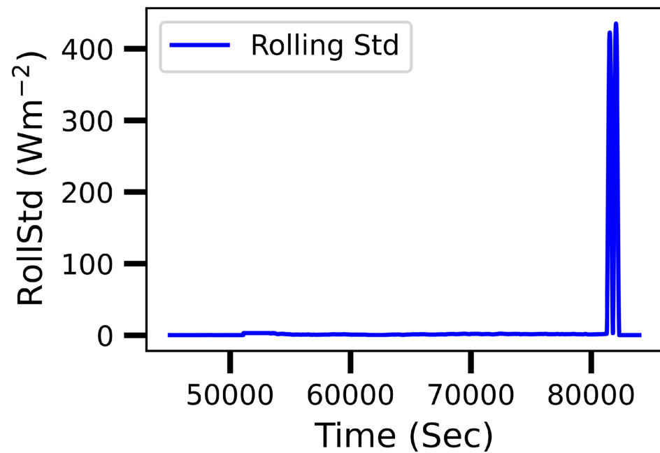
Figure 3. from Anoop Gavankar et al 2026 Astron. J. 171 doi:10.3847/1538-3881/ae11115 https://dx.doi.org/10.3847/1538-3881/ae11115 © 2025. The Author(s). Published by the American Astronomical Society.
