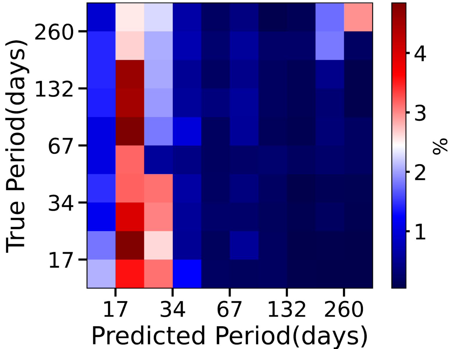
Figure 17. from Anoop Gavankar et al 2026 Astron. J. 171 doi:10.3847/1538-3881/ae11115 https://dx.doi.org/10.3847/1538-3881/ae11115 © 2025. The Author(s). Published by the American Astronomical Society.
