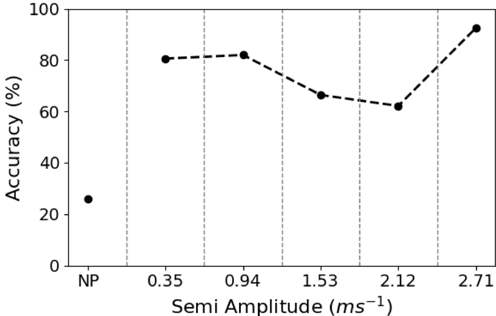
Figure 16. from Anoop Gavankar et al 2026 Astron. J. 171 doi:10.3847/1538-3881/ae11115 https://dx.doi.org/10.3847/1538-3881/ae11115 © 2025. The Author(s). Published by the American Astronomical Society.
