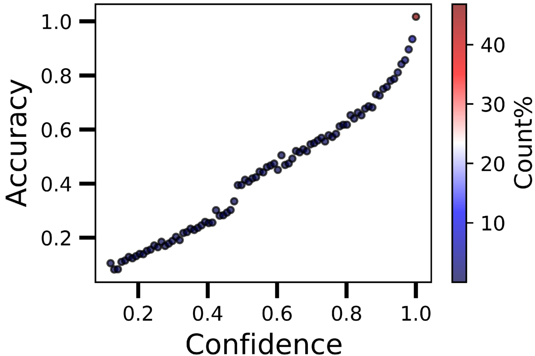
Figure 14. from Anoop Gavankar et al 2026 Astron. J. 171 doi:10.3847/1538-3881/ae11115 https://dx.doi.org/10.3847/1538-3881/ae11115 © 2025. The Author(s). Published by the American Astronomical Society.
