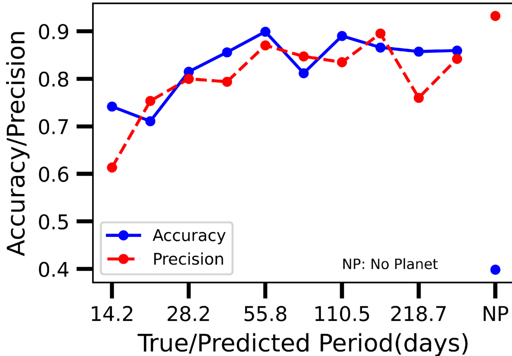
Figure 13. from Anoop Gavankar et al 2026 Astron. J. 171 doi:10.3847/1538-3881/ae11115 https://dx.doi.org/10.3847/1538-3881/ae11115 © 2025. The Author(s). Published by the American Astronomical Society.
