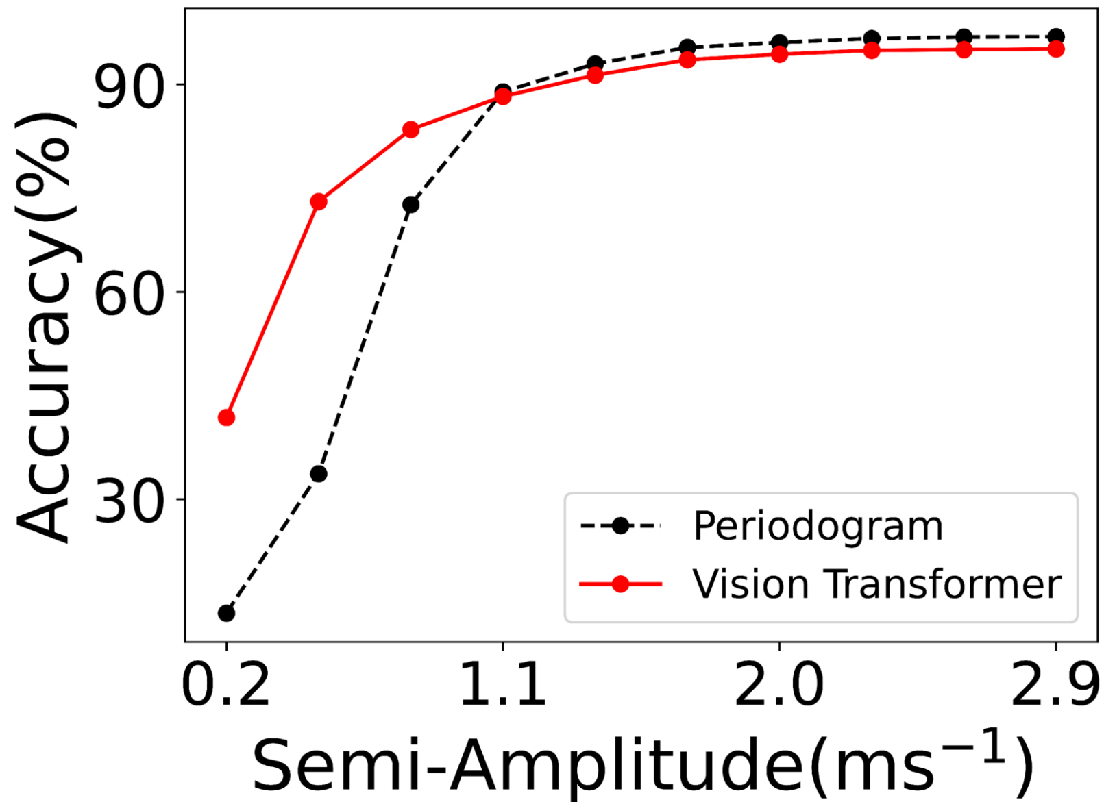
Figure 12. from Anoop Gavankar et al 2026 Astron. J. 171 doi:10.3847/1538-3881/ae11115 https://dx.doi.org/10.3847/1538-3881/ae11115 © 2025. The Author(s). Published by the American Astronomical Society.
