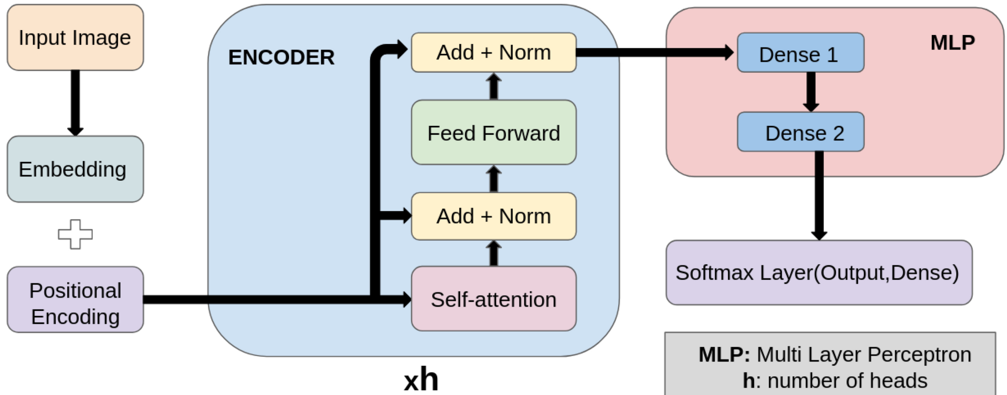
Figure 10. from Anoop Gavankar et al 2026 Astron. J. 171 doi:10.3847/1538-3881/ae1115 https://dx.doi.org/10.3847/1538-3881/ae1115 © 2025. The Author(s). Published by the American Astronomical Society.
