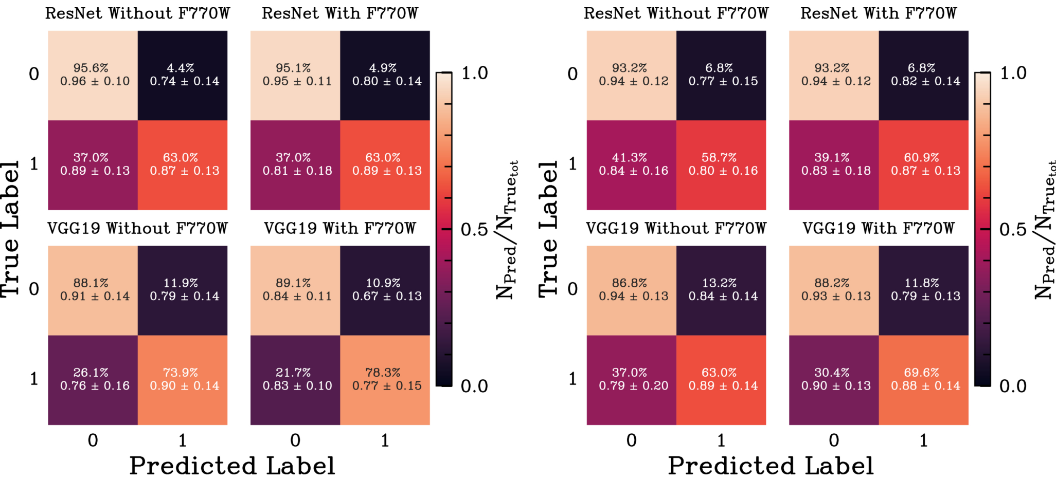
Figure 9. from Gabrielle B. Graham et al 2025 Astron. J. 170 doi:10.3847/1538-3881/ae10ad https://dx.doi.org/10.3847/1538-3881/ae10ad © 2025. The Author(s). Published by the American Astronomical Society.
