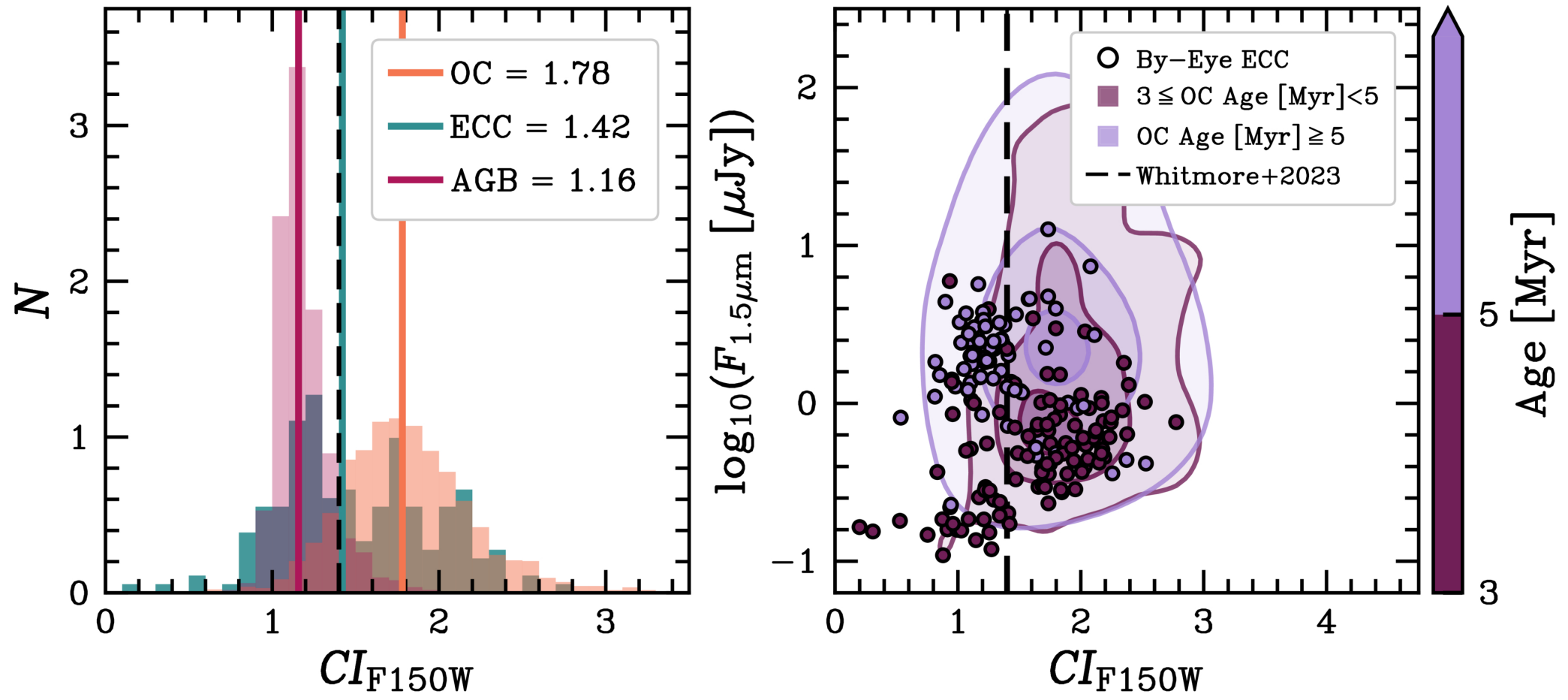
Figure 7. from Gabrielle B. Graham et al 2025 Astron. J. 170 doi:10.3847/1538-3881/ae10ad https://dx.doi.org/10.3847/1538-3881/ae10ad © 2025. The Author(s). Published by the American Astronomical Society.
