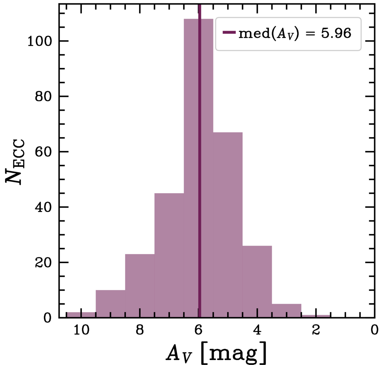
Figure 6. from Gabrielle B. Graham et al 2025 Astron. J. 170 doi:10.3847/1538-3881/ae10ad https://dx.doi.org/10.3847/1538-3881/ae10ad © 2025. The Author(s). Published by the American Astronomical Society.
