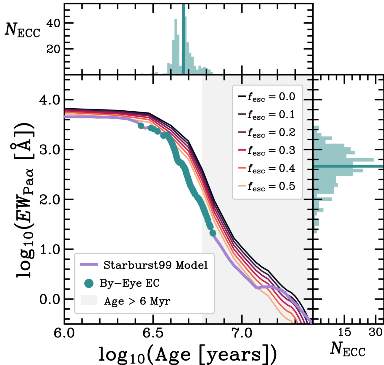
Figure 5. from Gabrielle B. Graham et al 2025 Astron. J. 170 doi:10.3847/1538-3881/ae10ad https://dx.doi.org/10.3847/1538-3881/ae10ad © 2025. The Author(s). Published by the American Astronomical Society.
