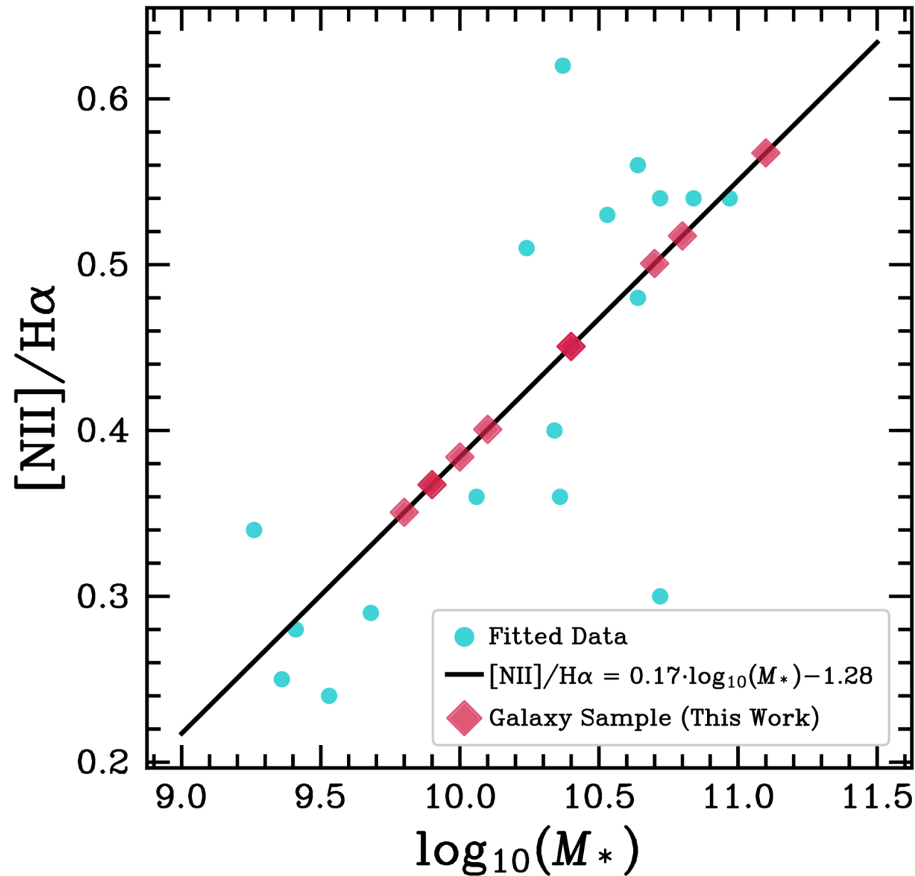
Figure 14. from Gabrielle B. Graham et al 2025 Astron. J. 170 doi:10.3847/1538-3881/ae10ad https://dx.doi.org/10.3847/1538-3881/ae10ad © 2025. The Author(s). Published by the American Astronomical Society.
