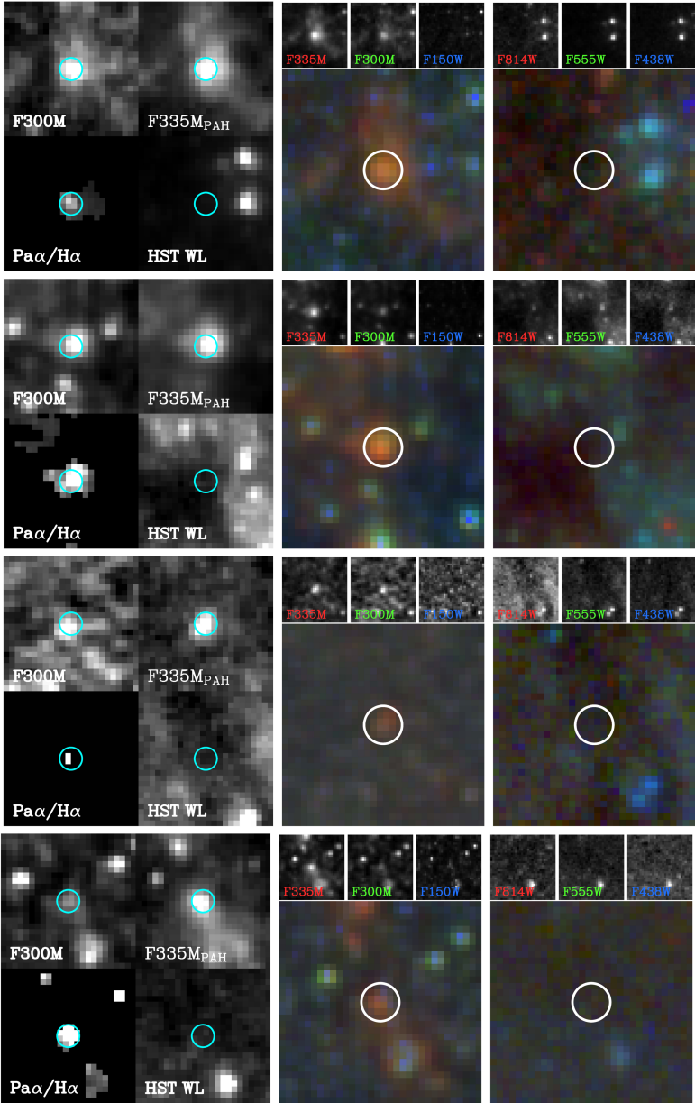
Figure 13. from Gabrielle B. Graham et al 2025 Astron. J. 170 doi:10.3847/1538-3881/ae10ad https://dx.doi.org/10.3847/1538-3881/ae10ad © 2025. The Author(s). Published by the American Astronomical Society.
