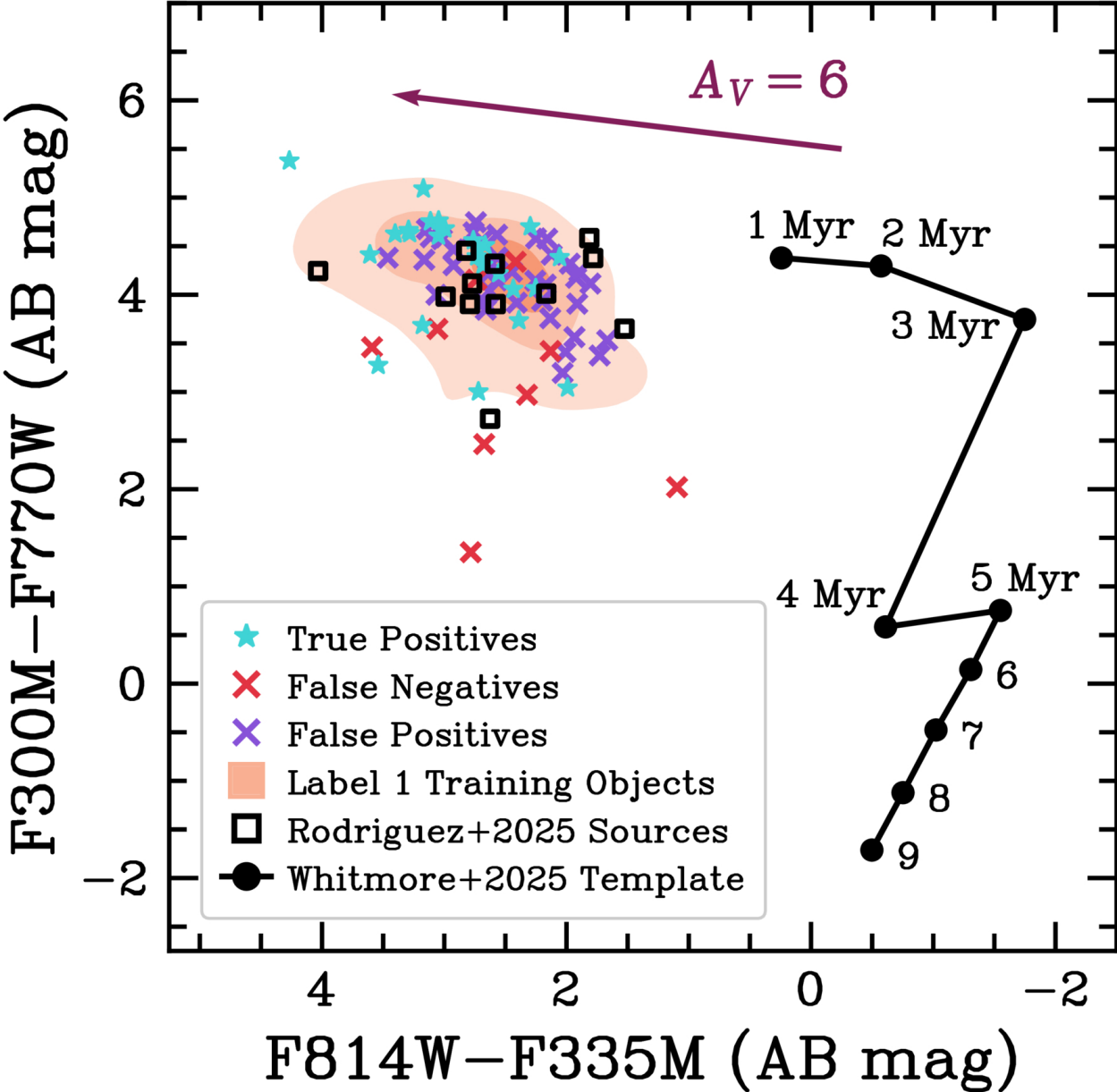
Figure 11. from Gabrielle B. Graham et al 2025 Astron. J. 170 doi:10.3847/1538-3881/ae10ad https://dx.doi.org/10.3847/1538-3881/ae10ad © 2025. The Author(s). Published by the American Astronomical Society.
