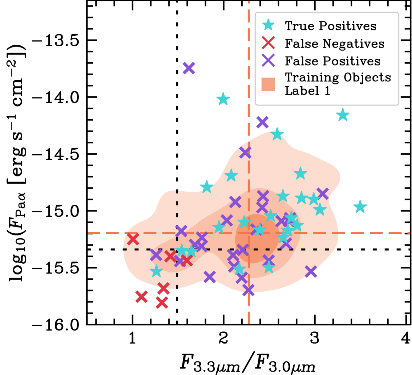
Figure 10. from Gabrielle B. Graham et al 2025 Astron. J. 170 doi:10.3847/1538-3881/ae10ad https://dx.doi.org/10.3847/1538-3881/ae10ad © 2025. The Author(s). Published by the American Astronomical Society.
