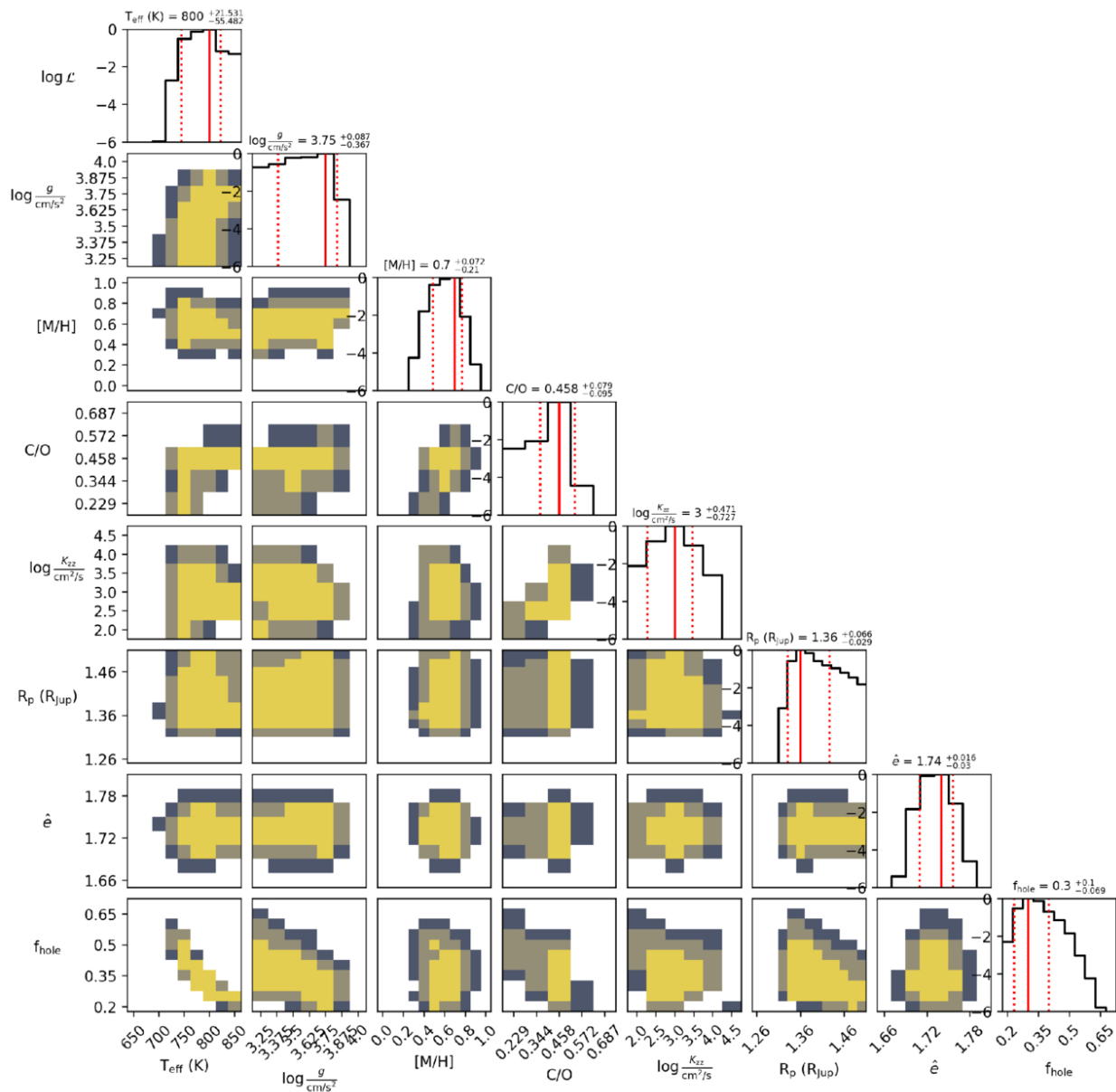
Figure 8. from Alexander Madurowicz et al 2025 Astron. J. 170 doi:10.3847/1538-3881/ae1028 https://dx.doi.org/10.3847/1538-3881/ae1028 © 2025. The Author(s). Published by the American Astronomical Society.
