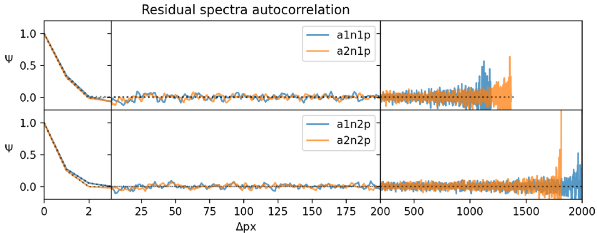
Figure 7. from Alexander Madurowicz et al 2025 Astron. J. 170 doi:10.3847/1538-3881/ae1028 https://dx.doi.org/10.3847/1538-3881/ae1028 © 2025. The Author(s). Published by the American Astronomical Society.
