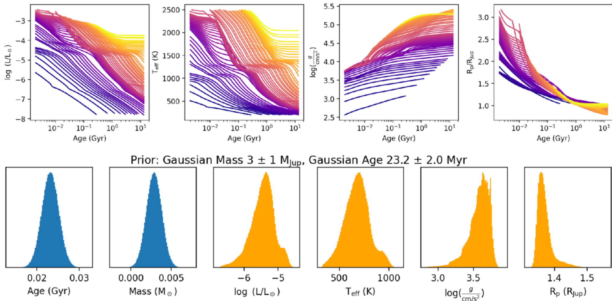
Figure 5. from Alexander Madurowicz et al 2025 Astron. J. 170 doi:10.3847/1538-3881/ae1028 https://dx.doi.org/10.3847/1538-3881/ae1028 © 2025. The Author(s). Published by the American Astronomical Society.
