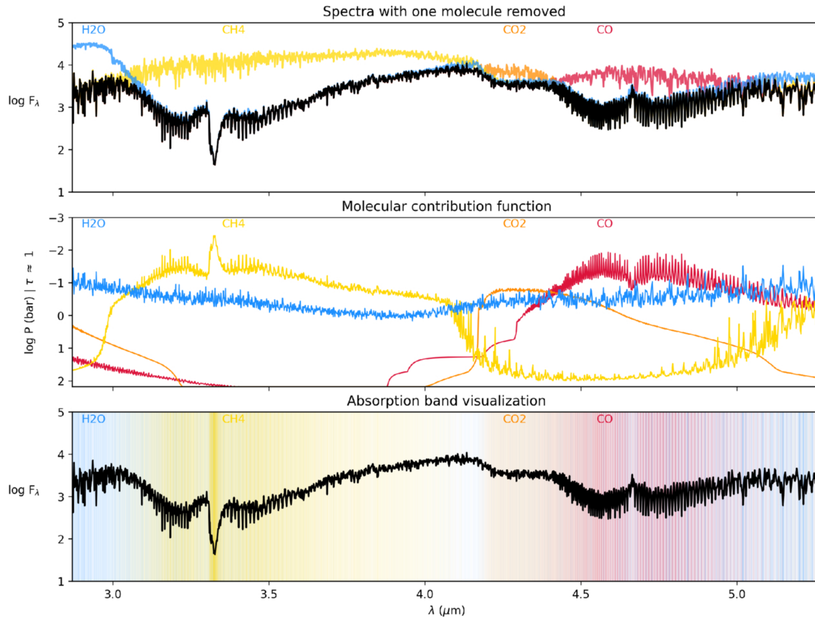
Figure 3. from Alexander Madurowicz et al 2025 Astron. J. 170 doi:10.3847/1538-3881/ae1028 https://dx.doi.org/10.3847/1538-3881/ae1028 © 2025. The Author(s). Published by the American Astronomical Society.
