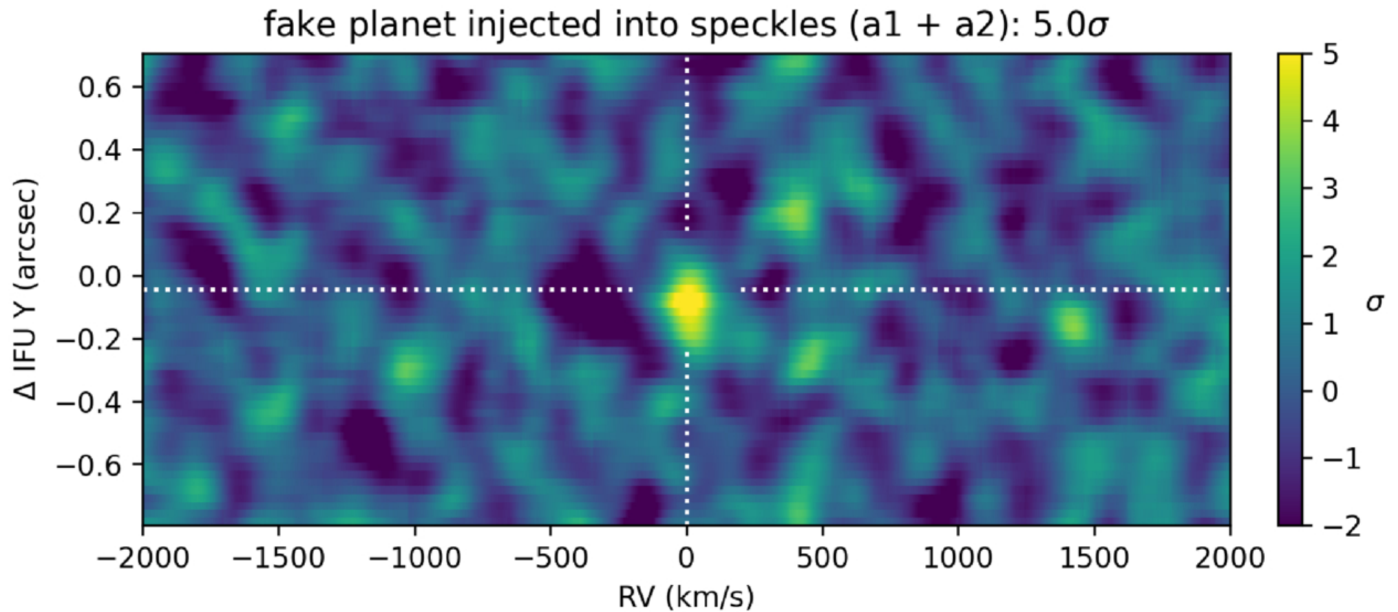
Figure 10. from Alexander Madurowicz et al 2025 Astron. J. 170 doi:10.3847/1538-3881/ae1028 https://dx.doi.org/10.3847/1538-3881/ae1028 © 2025. The Author(s). Published by the American Astronomical Society.
